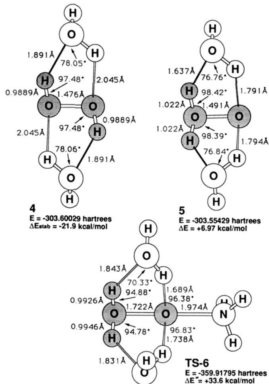
Figure 3. Hydrogen peroxide ( 4 ) and water oxide ( 5 ) hydrogen bonded to two water molecules and the transition state for oxygen atom transfer from water oxide complex 5 to ammonia (TS-6). Geometries were fully optimized at the MP2/6-31G* level, relative energies (MP4//MP2/6-31G*) for 4 and 5 are measured from isolated \text{H}_2\text{O}_2 and two water molecules, and the barrier for TS-6 is computed relative to the reactant cluster with hydrogen peroxide 4 . The total energies for \text{NH}_3 , \text{H}_2\text{O} , \text{H}_2\text{O}_2 , and \text{H}_2\text{OO} are -56.371\ 26 , -76.207\ 33 , -151.150\ 74 , and -151.071\ 56 au, respectively.
