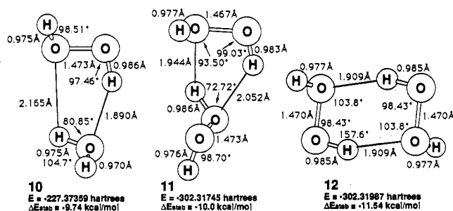
Figure 5. Hydrogen bonded complexes of hydrogen peroxide. Geometries are at MP2/6-31G*, and energies are at MP4/6-31G**/MP2/6-31G*.
