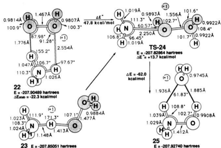
Figure 10. Optimized geometries of the complex of \text{H}_2\text{O}_2 with \text{NH}_4^+ ( \mathbf{22} ), \text{NH}_3 with \text{HO}^+\text{-OH}_2 ( \mathbf{23} ), the transition state for oxygen atom transfer from the hydroperoxonium ion to ammonia (TS-24), and the reaction product ( \mathbf{25} ). Geometries are at MP2/6-31G*, and energies are at MP4//MP2/6-31G*. The total energies of \text{NH}_3 , \text{NH}_4^+ , and \text{HO-OH}_2 are -56.371\ 26 , -56.718\ 61 , and -151.417\ 60 au, respectively.
