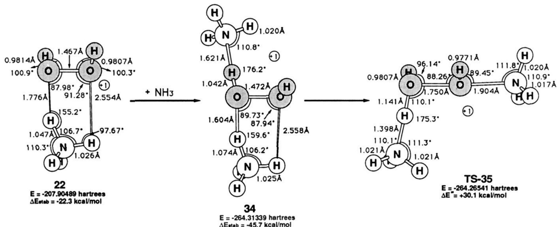
Figure 14. Concerted oxygen atom transfer from hydrogen peroxide to ammonia catalyzed by the ammonium ion. Geometries are at MP2/6-31G*, and energies are at MP4//MP2/6-31G*. The total energy is NH 3 is -56.371 26 au.
