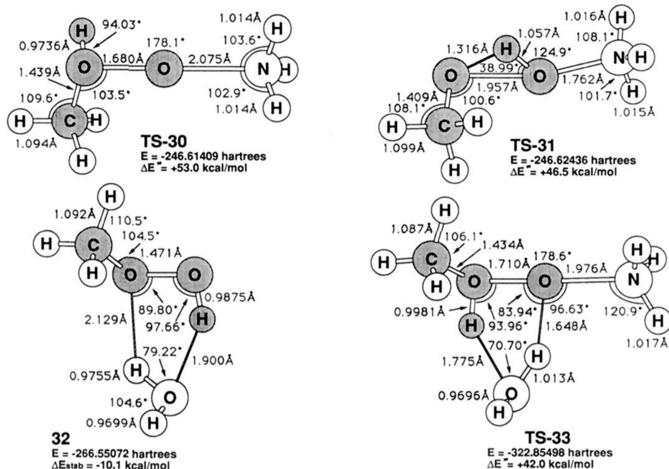
Figure 12. Transition structures for oxygen atom transfer from methyl hydroperoxide with proton transfer before (TS-30) and after (TS-31) oxygen atom transfer with (TS-33) and without (TS-31) water catalysis. Geometries were calculated at MP2/6-31G* and barriers at MP4/6-31G*/MP2/6-31G*. The total energy of CH 3 OOH is -190.327 24 au.
