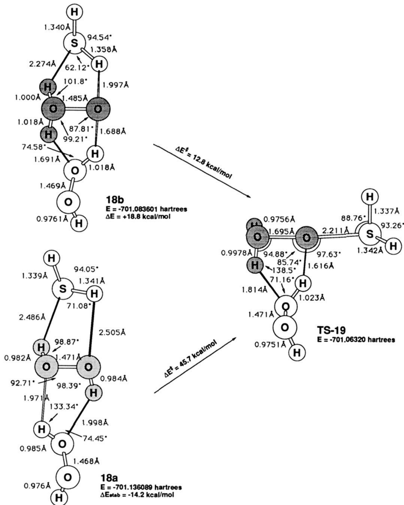
Figure 7. Oxygen atom transfer from hydrogen peroxide dimer to H 2 S. Geometries are at MP2/6-31G*, and energies are at MP4/6-31G**/MP2/6-31G*. The total energy of H 2 S is -398.812 00 au.
