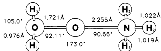
Figure 1. Transition structure (TS-1) for oxygen transfer from water oxide to ammonia. Geometry fully optimized at the QCISD(T)/6-31G* level.
