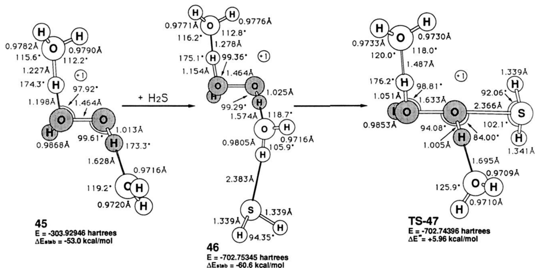
Figure 18. Oxidation of H 2 S by H 2 O 2 with H 3 O + catalysis and H 2 O stabilization of H 2 SOH + . Geometries are at MP2/6-31G*, and energies are at MP4//MP2/6-31G*.
