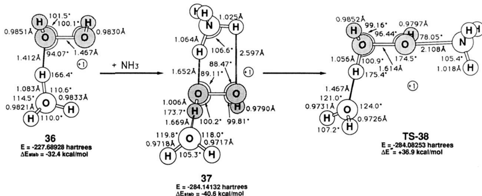
Figure 15. Hydronium ion catalyzed oxygen atom transfer from hydrogen peroxide to ammonia. Geometries are at MP2/6-31G*, and energies are at MP4//MP2/6-31G*. The total energies of H 3 O + , NH 3 , and H 2 O 2 are -76.486 87, -56.371 26, and -151.150 74 au, respectively.
