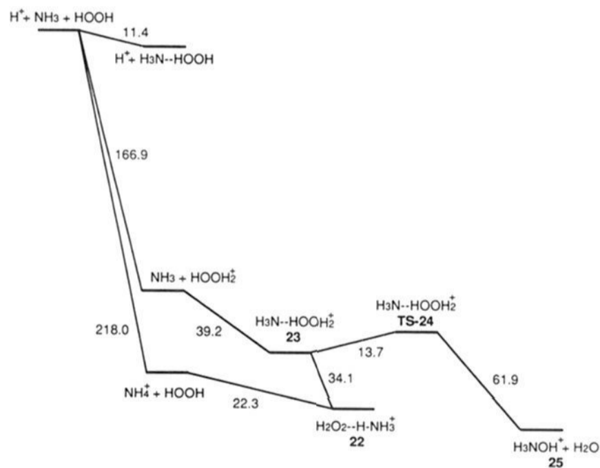
Figure 9. Relative energies (MP4//MP2/6-31G*) for the complexation of ammonium ion with hydrogen peroxide and the hydroxylation of ammonia by hydroperoxonium ion.
