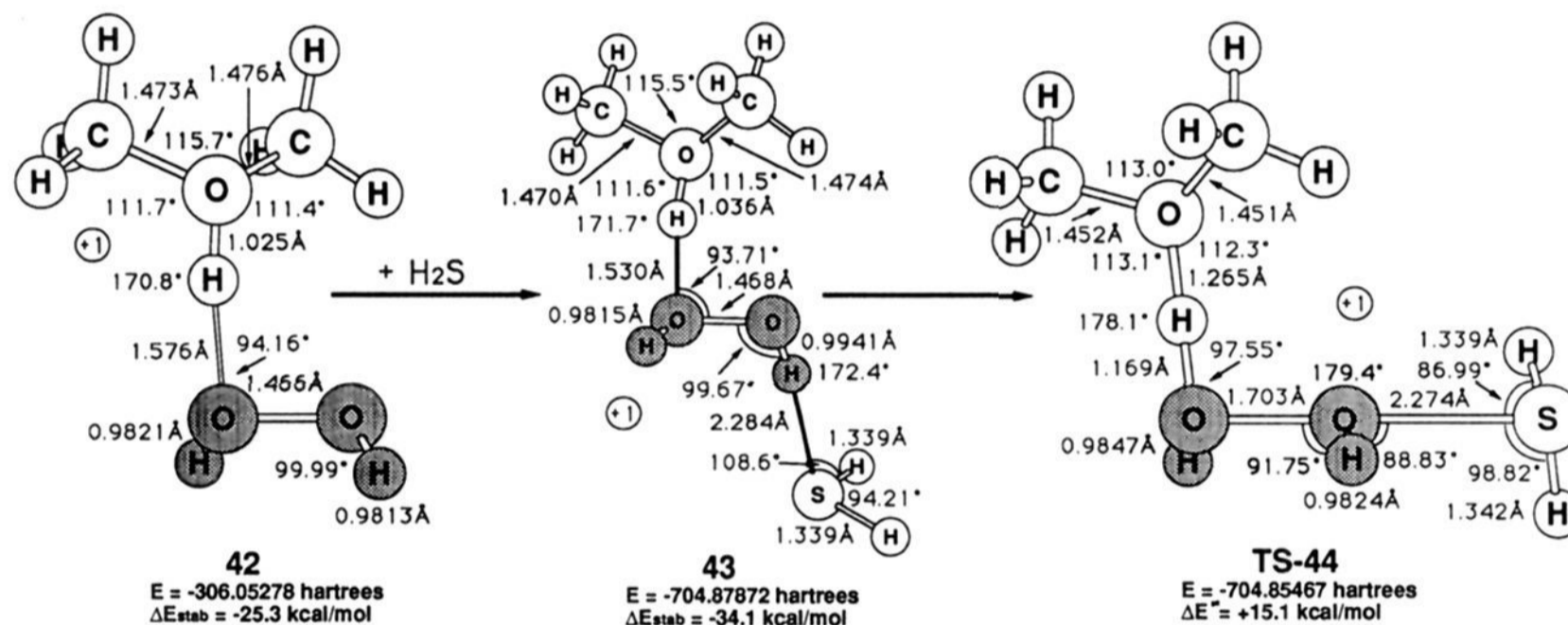
Figure 17. Oxygen atom transfer to dihydrogen sulfide catalyzed by dimethyl ether oxonium ion. Geometries are at MP2//MP2/6-31G*, and energies are at MP4//MP2/6-31G*. The total energies for (\text{CH}_3)_2\text{OH}^+ , \text{H}_2\text{O}_2 , and \text{H}_2\text{S} are -154.86165 , -151.15074 , and -398.81200 au, respectively.
