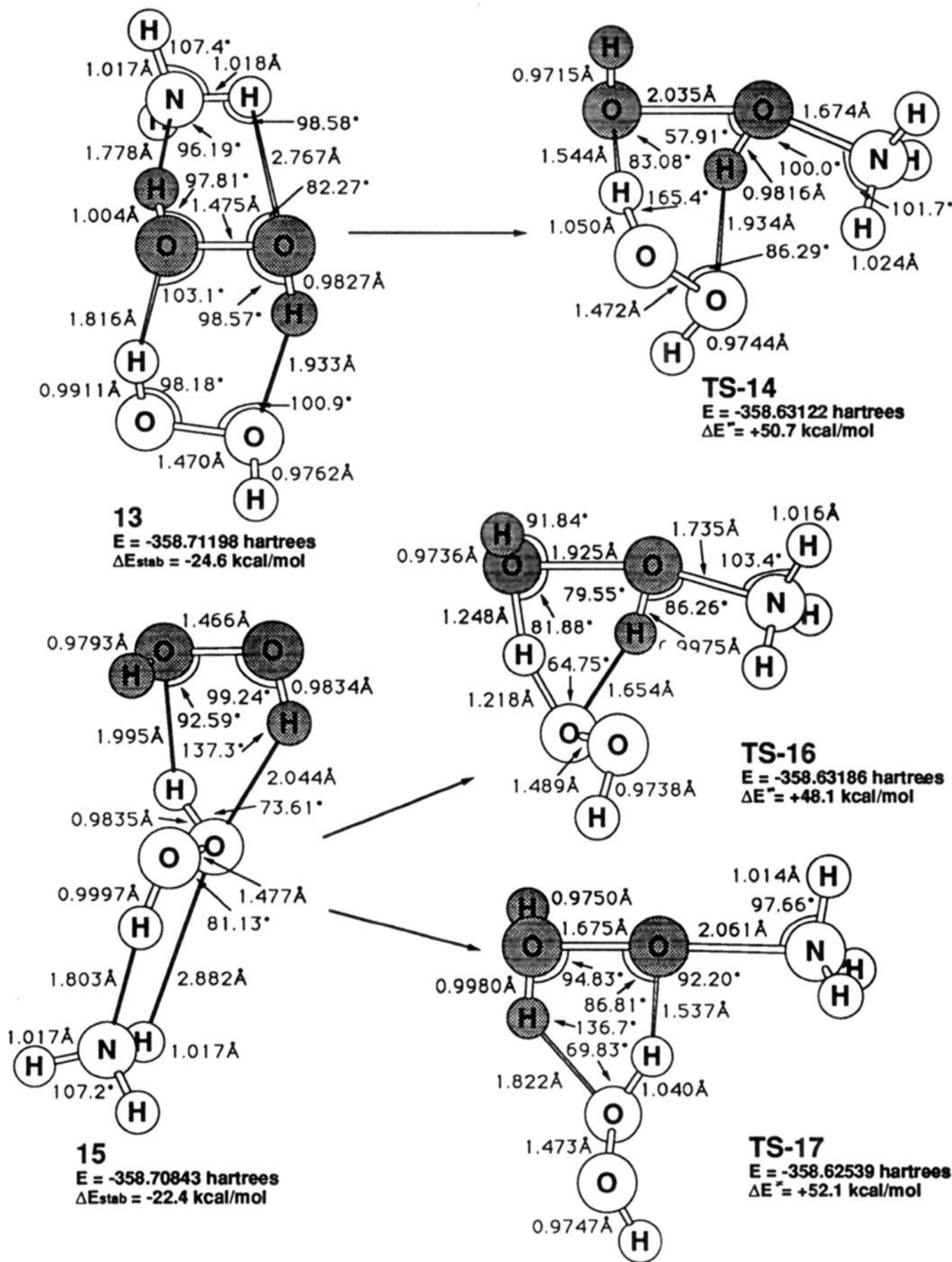
Figure 6. Optimized geometries for reactant clusters 13 and 15 and the transition structures for oxygen atom transfer from hydrogen peroxide dimer (TS-14, TS-16) and water oxide (TS-17) complexed to a molecule of hydrogen peroxide ammonia.
