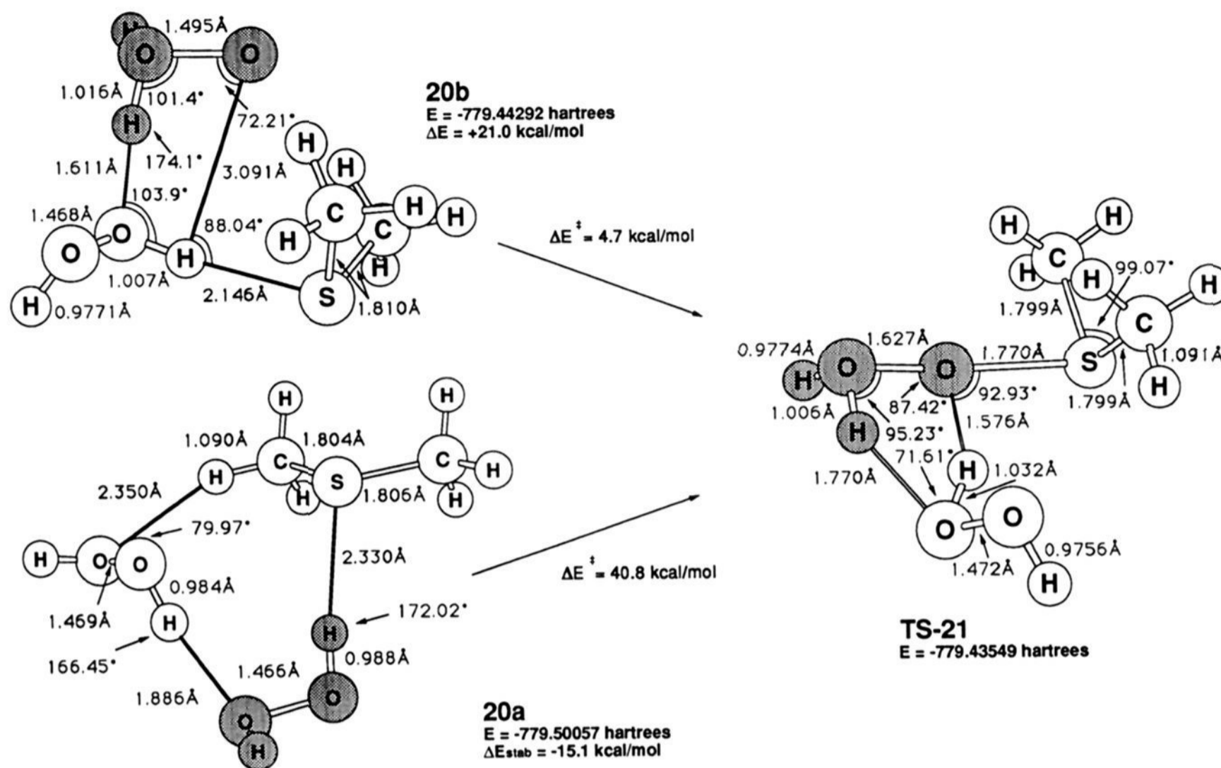
Figure 8. Oxygen atom transfer from hydrogen peroxide dimer to (\text{CH}_3)_2\text{S} . Geometries are at MP2/6-31G*, and energies are at MP4/6-31G*//MP2/6-31G*. The total energy of (\text{CH}_3)_2\text{S} is 477.174 987 au.
