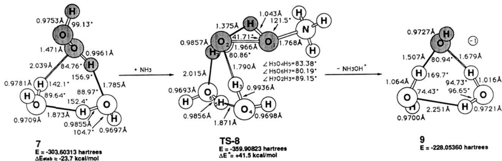
Figure 4. Ionic pathway for oxygen atom transfer from hydrogen peroxide catalyzed by two water molecules. Geometries are at MP2/6-31G*, and energies are at MP4//MP2/6-31G*. The activation energy ( \Delta E^\ddagger ) is computed relative to isolated \text{NH}_3 and hydrogen bonded complex 7 . The MP4//MP2/6-31G* energy of \text{NH}_3 is -56.37\ 26 au.
