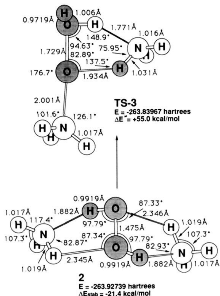
Figure 2. Oxygen atom transfer from hydrogen peroxide to ammonia catalyzed by one molecule of ammonia. Geometries are at MP2/6-31G*, and energies are at MP4/6-31G*//MP2/6-31G*.
