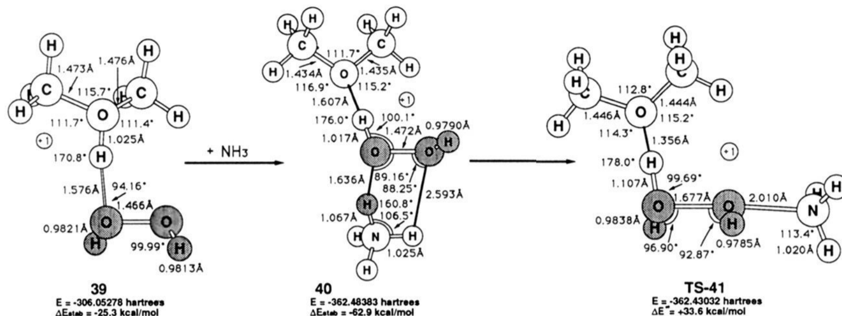
Figure 16. Concerted oxygen atom transfer from hydrogen peroxide to ammonia catalyzed by ammonium and dimethyl ether oxonium ions. Geometries are at MP2/6-31G*, and energies are at MP4//MP2/6-31G*.
