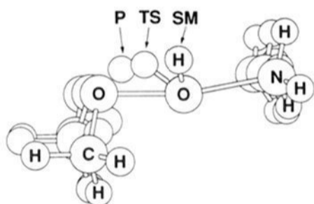
Figure 13. Three points along the reaction path for oxidation of ammonia by methyl hydroperoxide by the reaction path following the algorithm at the MP2/6-31G* level of theory: SM, a point along the reaction path from starting materials; TS, transition state (TS-31); P, a point on the reaction path toward the products.
