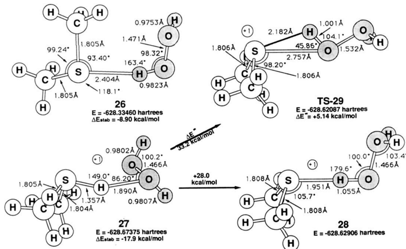
Figure 11. Oxygen atom transfer from protonated hydrogen peroxide to dimethyl sulfide. Geometries are at MP2/6-31G*, and energies are at MP4//MP2/6-31G*. The total energies of (\text{CH}_3)_2\text{S} , (\text{CH}_3)_2\text{SH}^+ , and \text{H}_2\text{O}_2 are -477.16968 , -477.49451 , and -151.15074 au, respectively.
